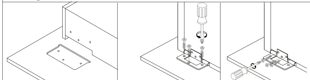
Fixings Pack #5-3
