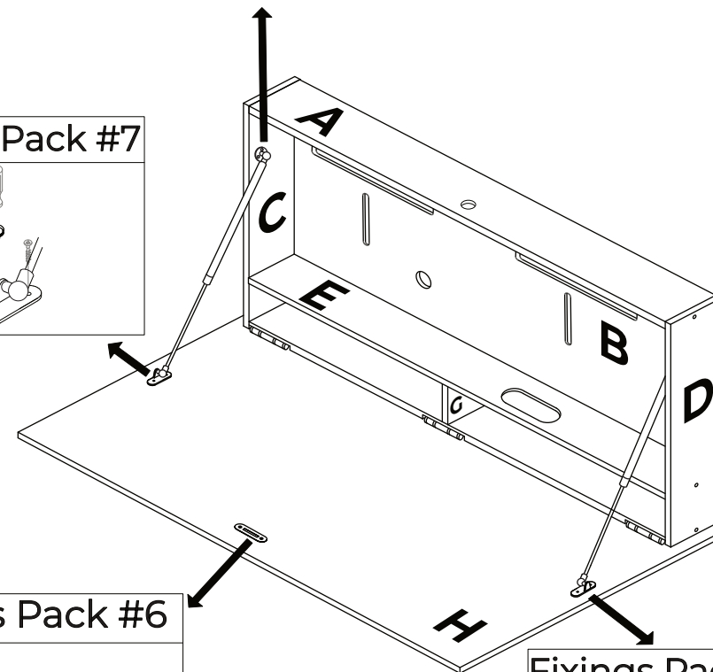
Fixings Pack #7
